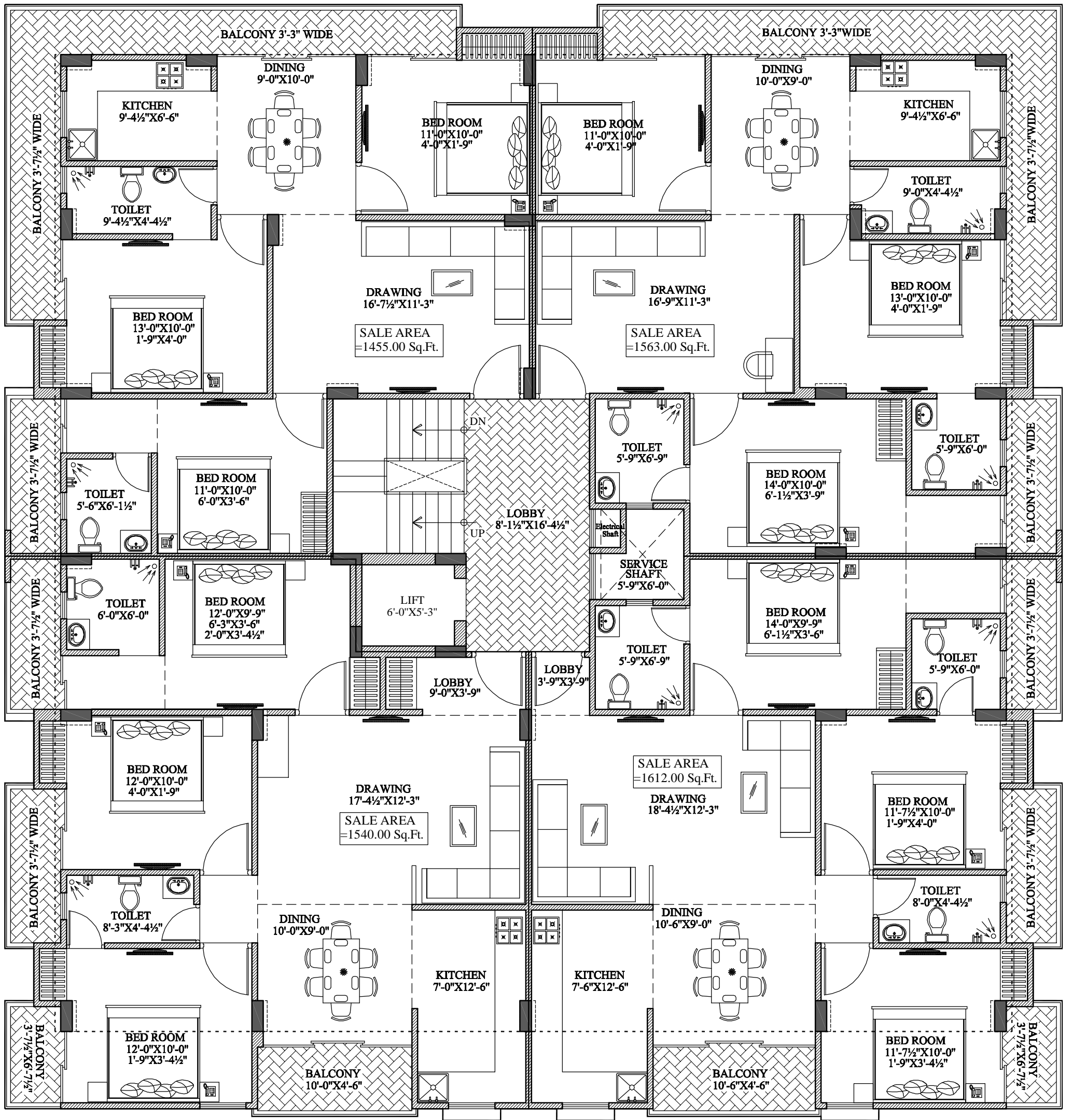
TYPICAL 1ST TO 4TH FLOOR PLAN
